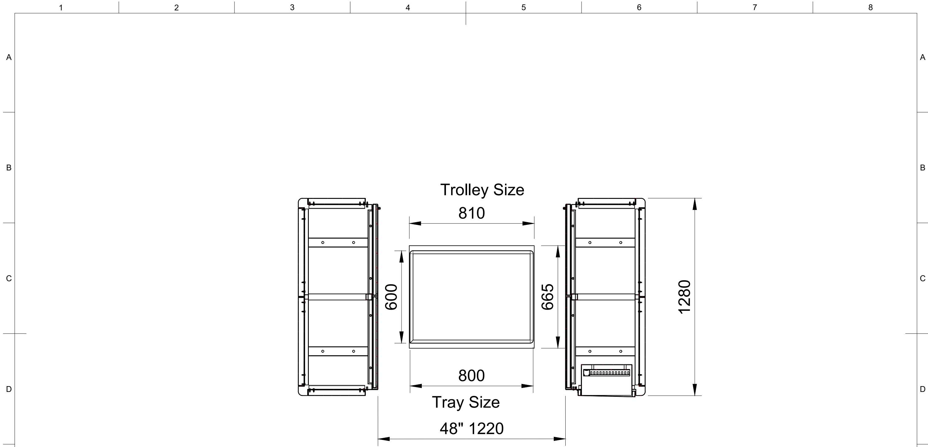
Section Plan (1:15)
